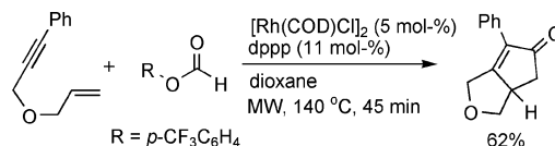
Scheme 2. Microwave-assisted cascade decarbonylation–Pauson–Khand-type reaction with the use of formate as a CO surrogate; under conventional oil-bath heating, 3 d were required for completion of the reaction with 43% isolated yield.
