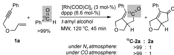
Scheme 1. Labeling experiment for microwave-assisted sequential CO-transfer process.
